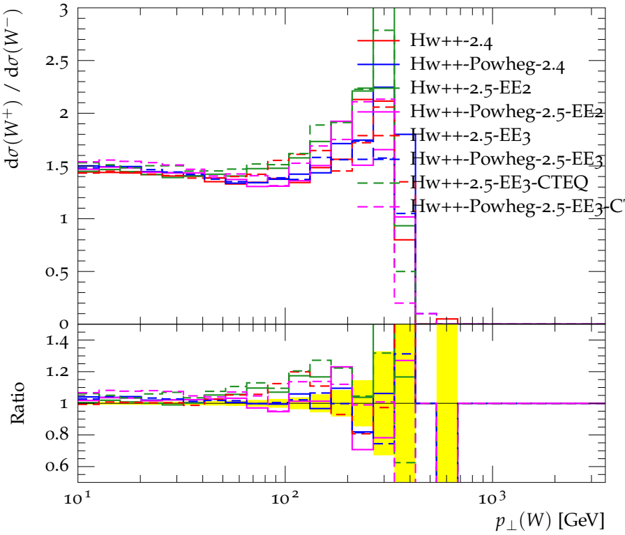
Charge asymmetry vs. p_{\perp}(W)
