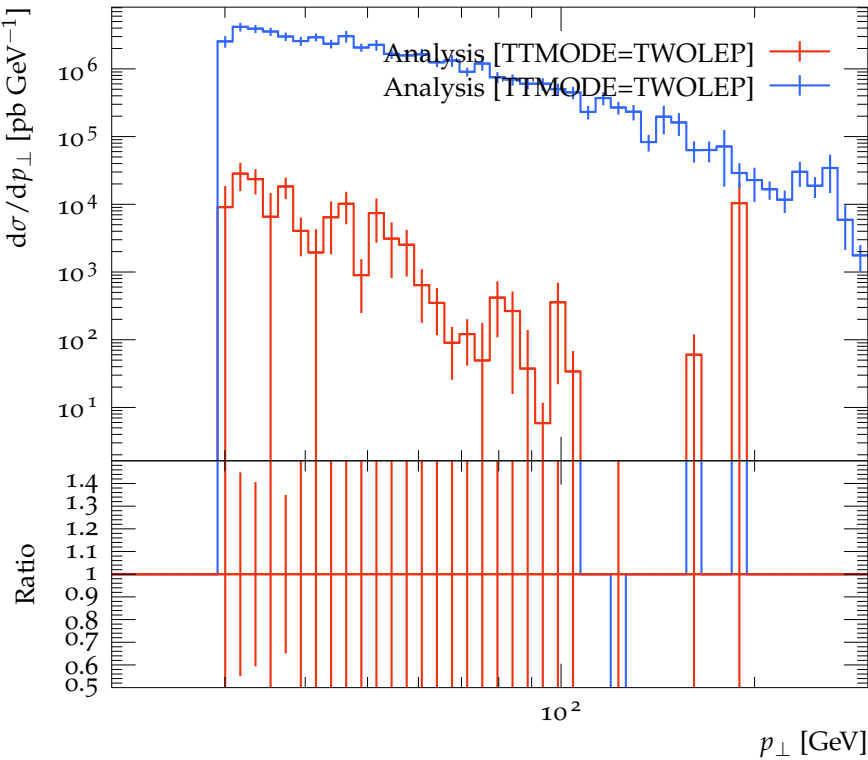
Transverse momentum distribution for light jet 2 ( N_\ell = 2 )
