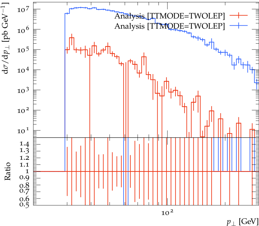
Transverse momentum distribution for jet 3
