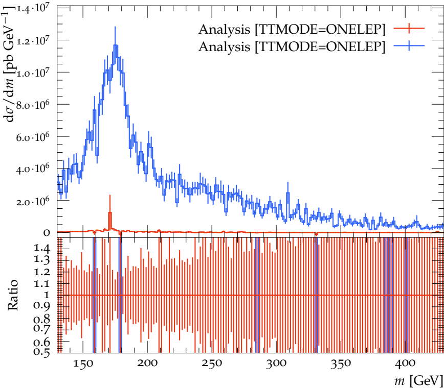
Mass distribution for reconstructed top after m_W cut ( N_\ell = 1 )
