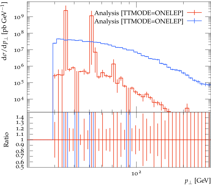
Transverse momentum distribution for light jet 2
