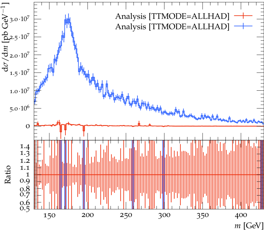
Mass distribution for reconstructed top after m_W cut ( N_\ell = 0 )
