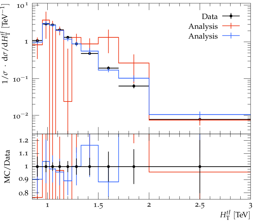
Particle-level t\bar{t} H_T
