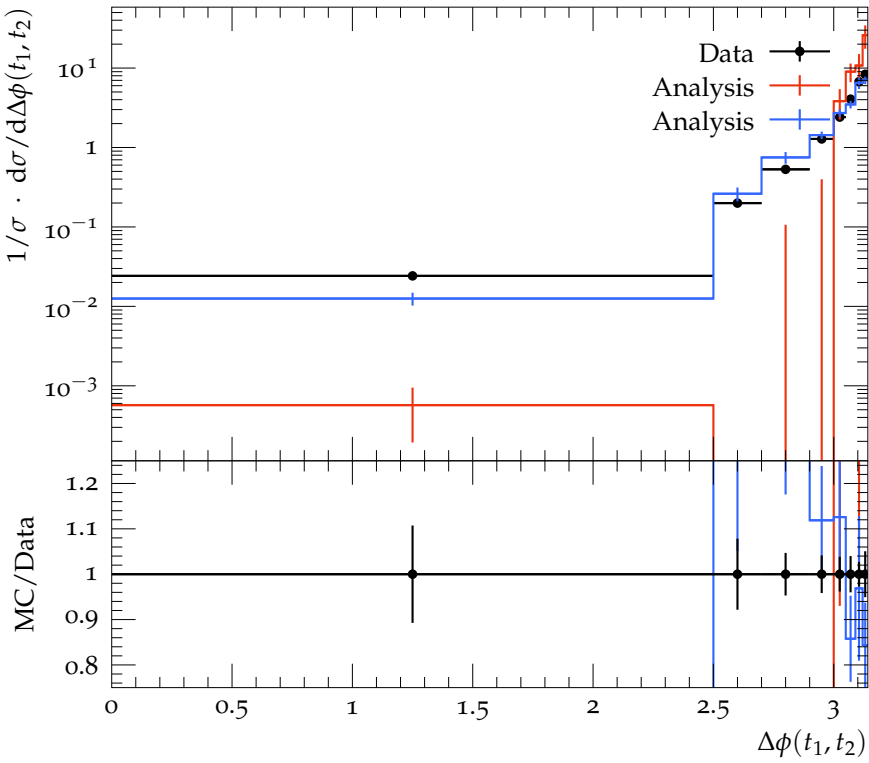
Particle-level t\bar{t} azimuthal opening angle
