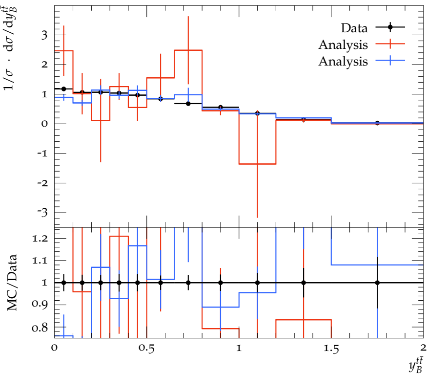
Particle-level t\bar{t} longitudinal boost
