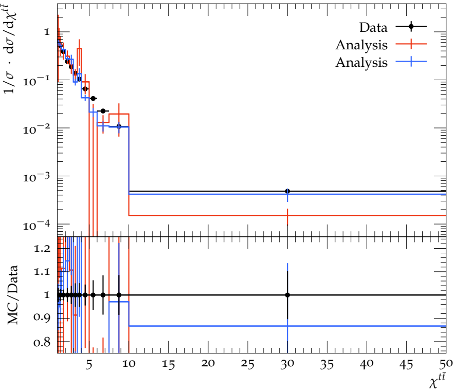
Particle-level t\bar{t} \chi
