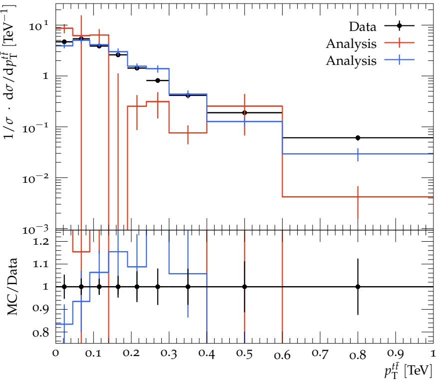
Particle-level t\bar{t} transverse momentum
