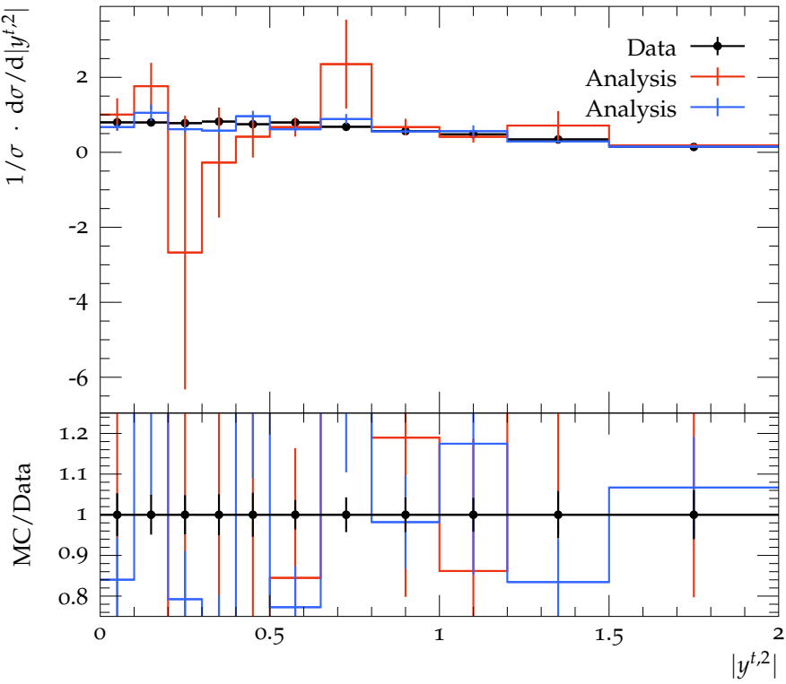
Particle-level subleading top rapidity
