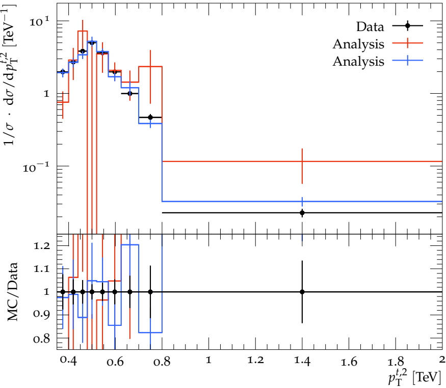
Particle-level subleading top transverse momentum
