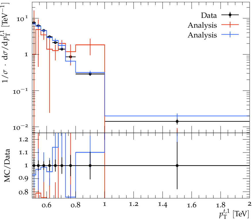
Particle-level leading top transverse momentum
