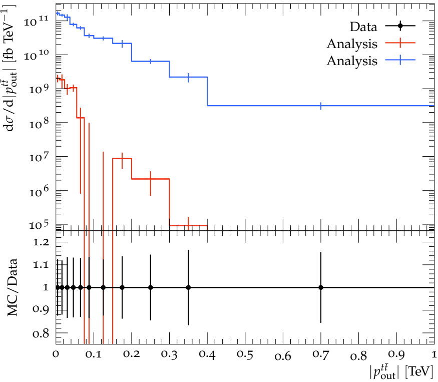
Particle-level t\bar{t} out-of-plane momentum
