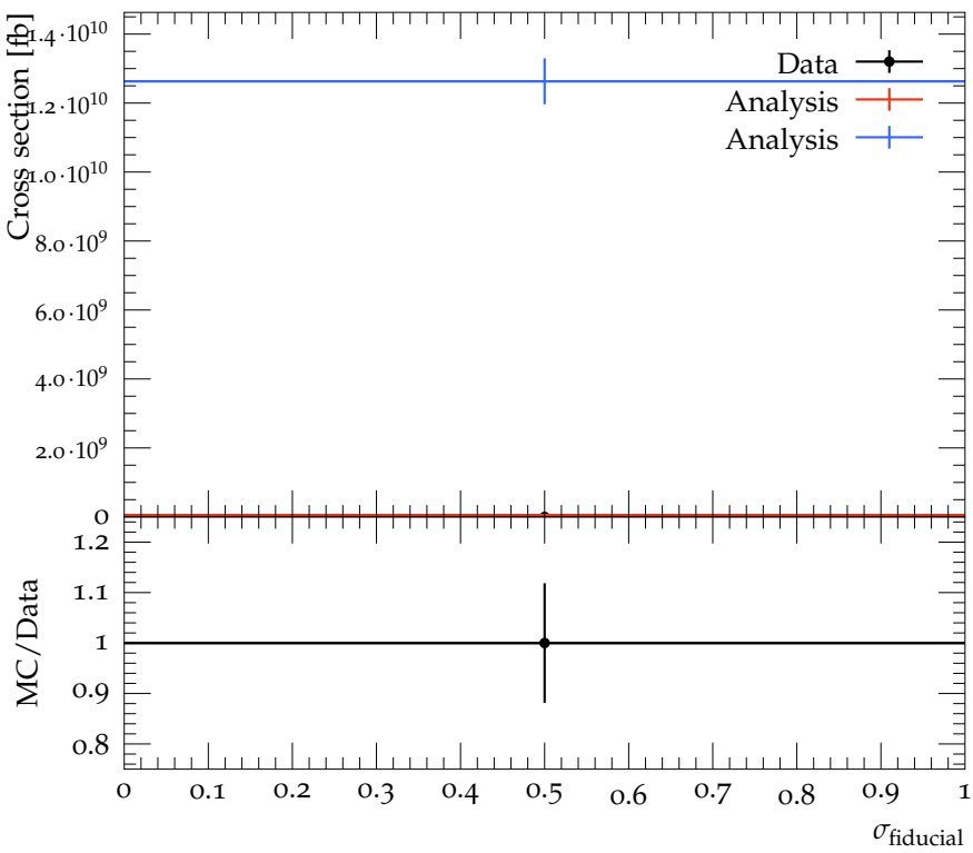
Particle-level fiducial phase-space total cross section
