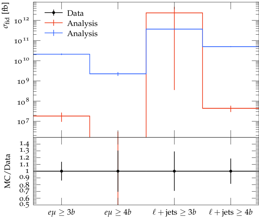
Fiducial cross-sections ( t\bar{t}X subtracted)
