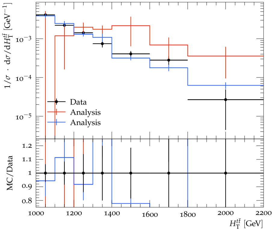
Particle-level t\bar{t} H_T
