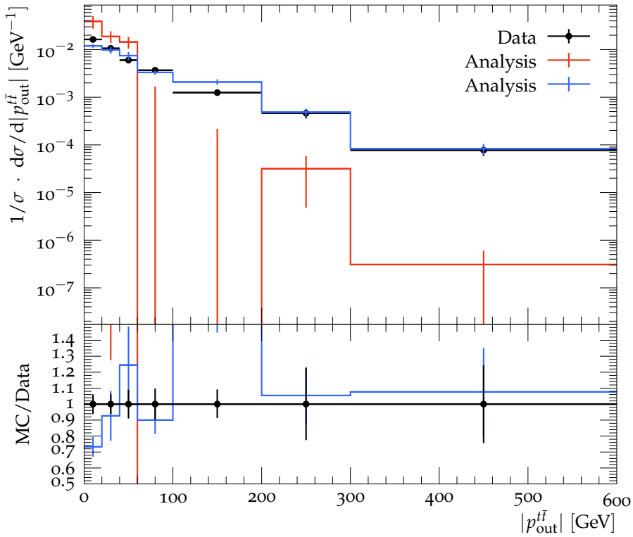
Particle-level t\bar{t} out-of-plane momentum
