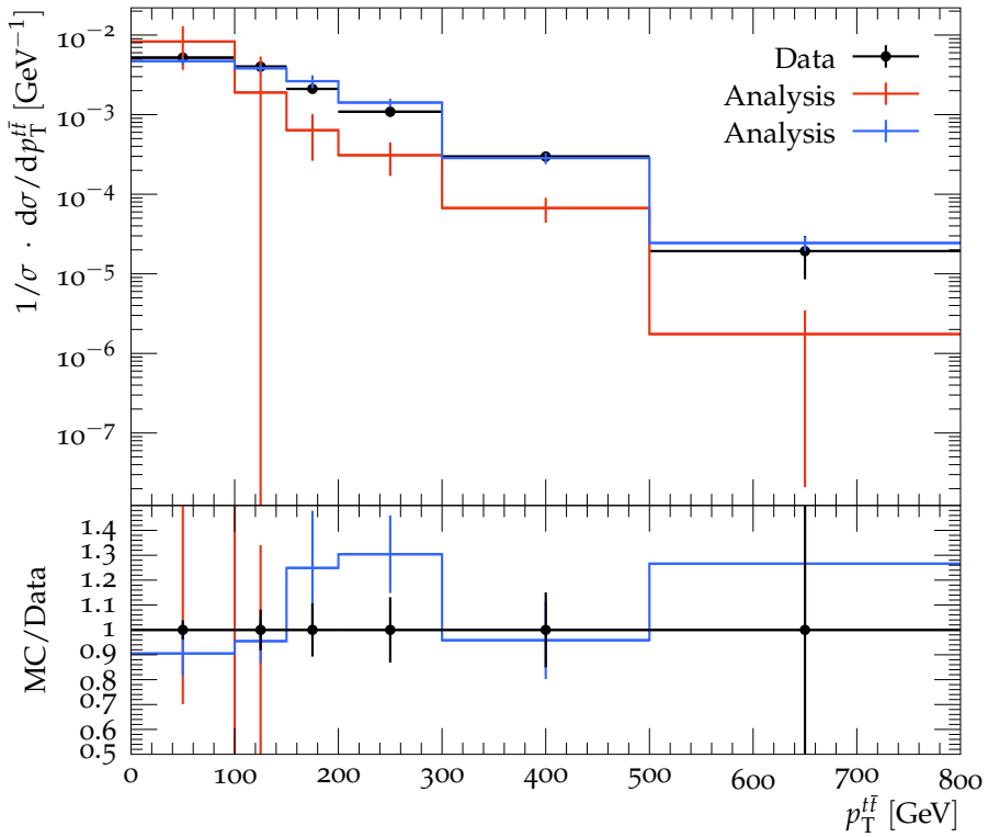
Particle-level t\bar{t} transverse momentum
