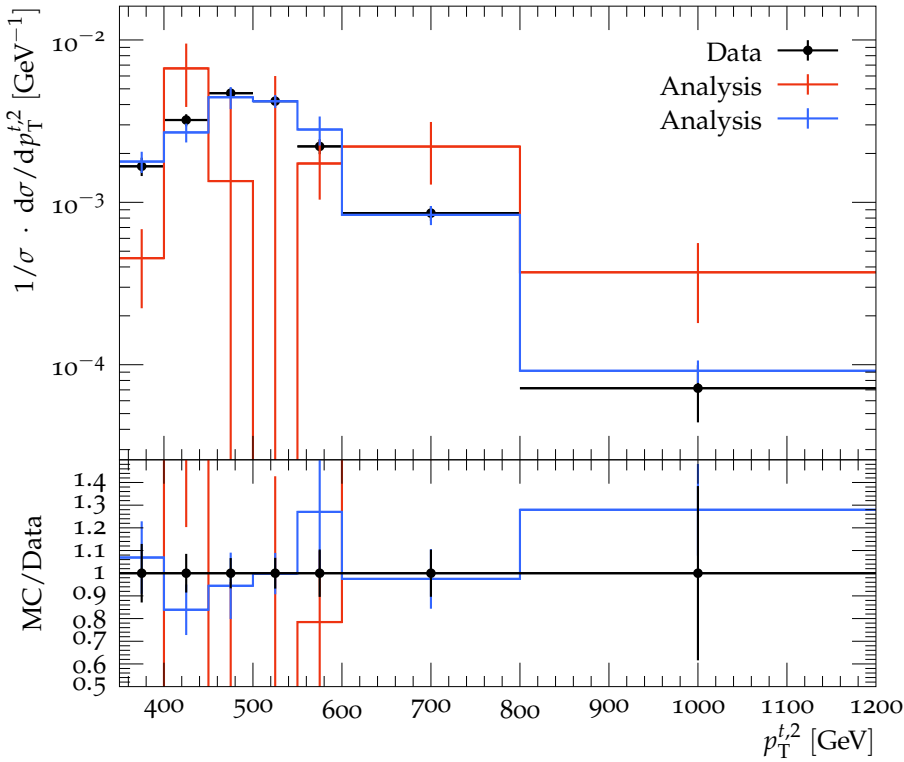
Particle-level subleading top transverse momentum
