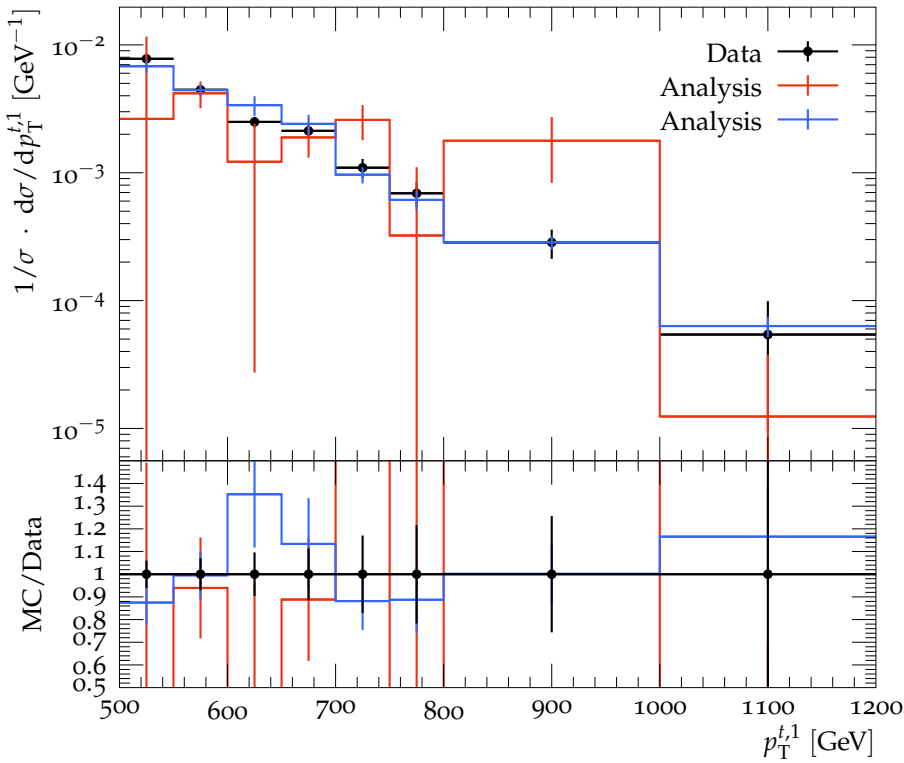
Particle-level leading top transverse momentum
