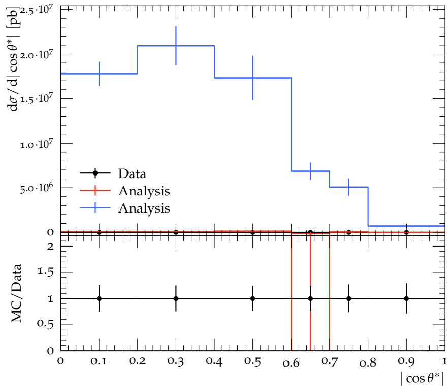
Particle-level t\bar{t} \cos \theta^*
