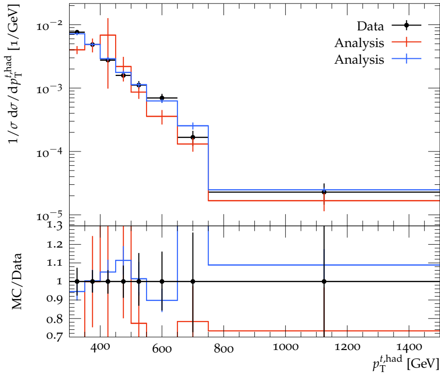
Combined lepton channels, boosted
