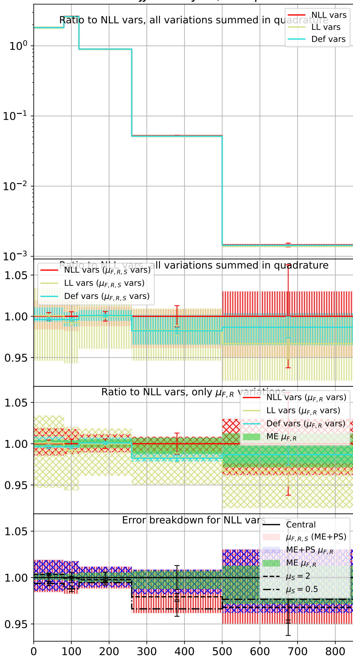
HISTO-PTH-DYJJ-5-6-PTJ-30, Sherpa default PS
