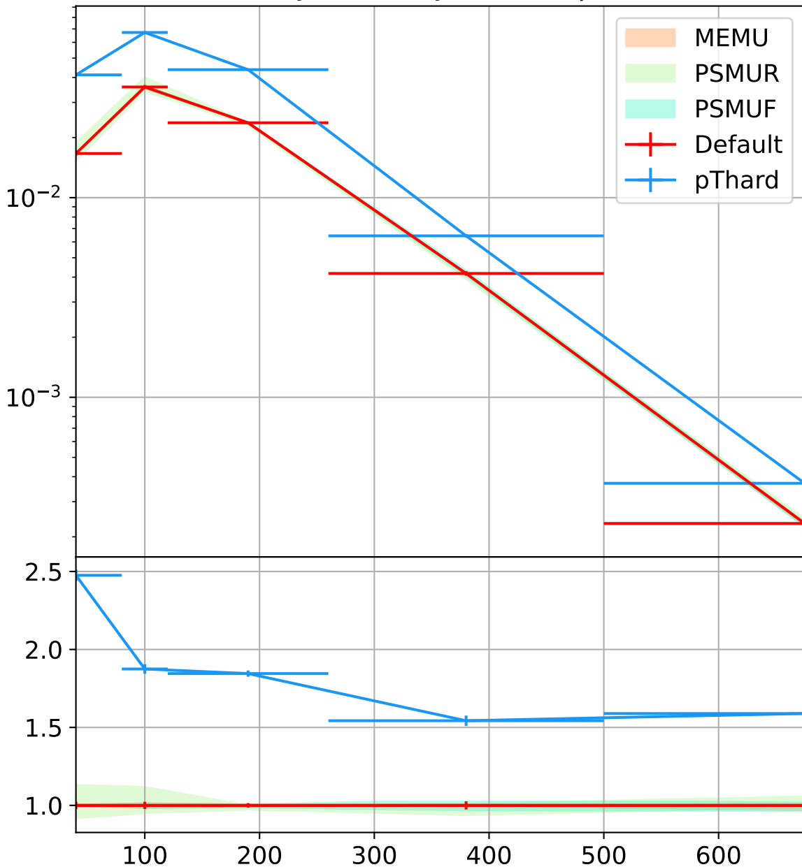
HISTO-PTH-NJETS-5-PTJ-20, Sherpa default PS
