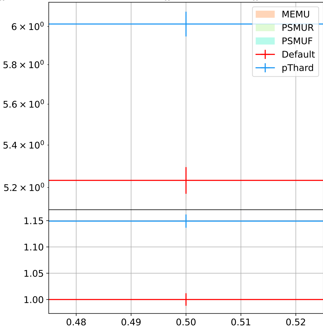
STXS-MJJ-350-700-PTH-200-INFTY-PTHJJ-25-INFTY-DPHIJJ-Plov2-PI, Sherpa default PS
