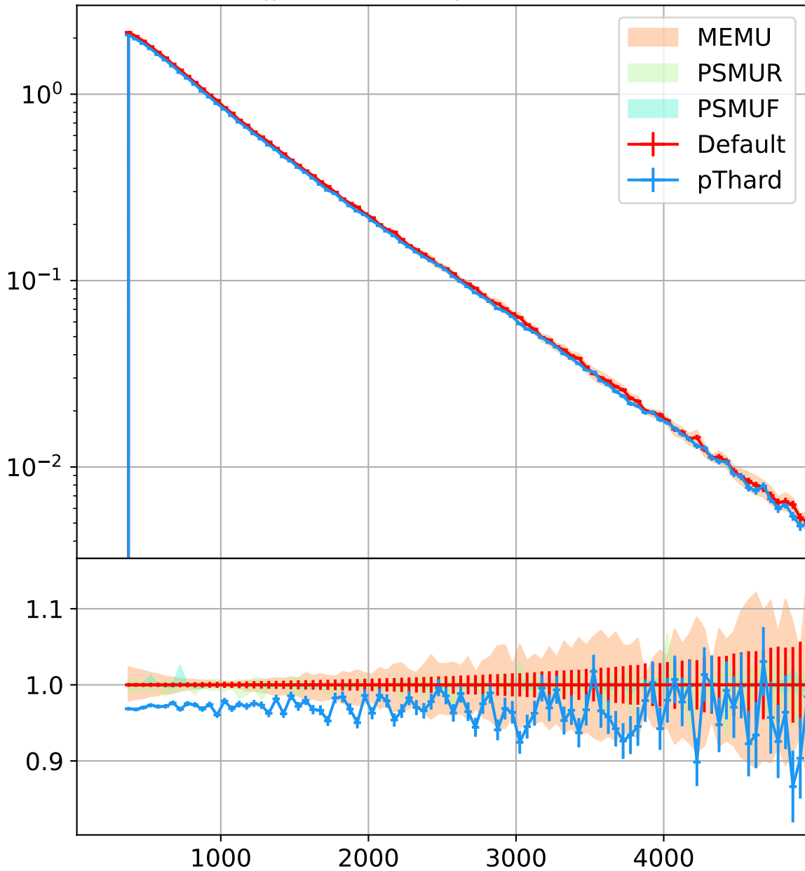
mjj-STXS, Sherpa default PS
