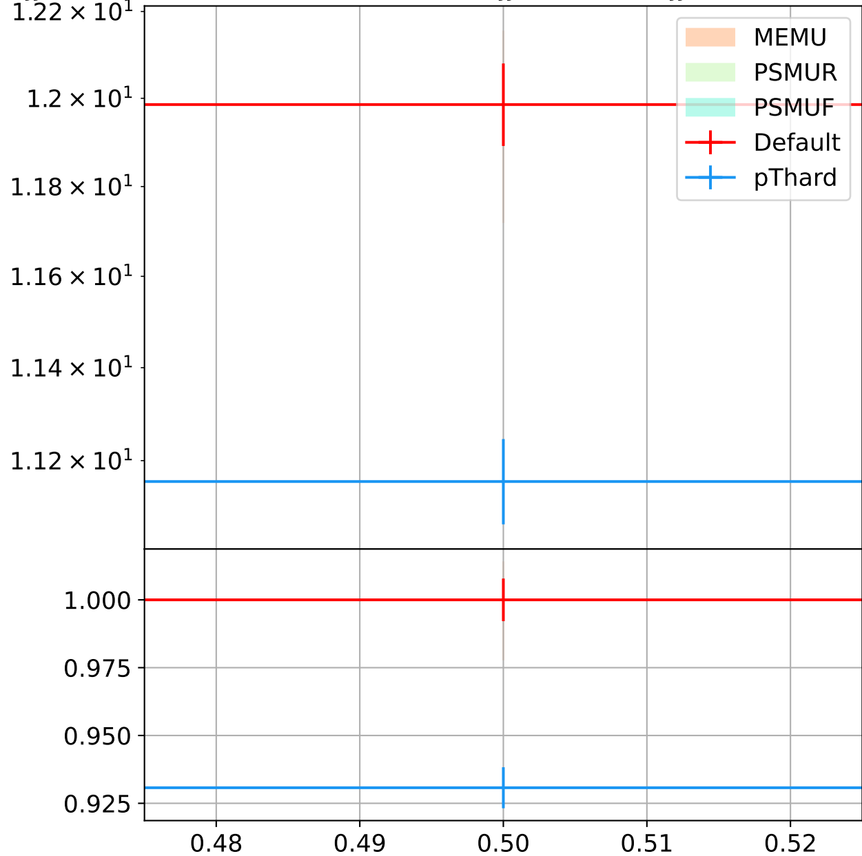
STXS-MJJ-1500-INFTY-PTH-200-INFTY-PTHJJ-0-25-DPHIJJ-Plov2-PI, Sherpa default PS
