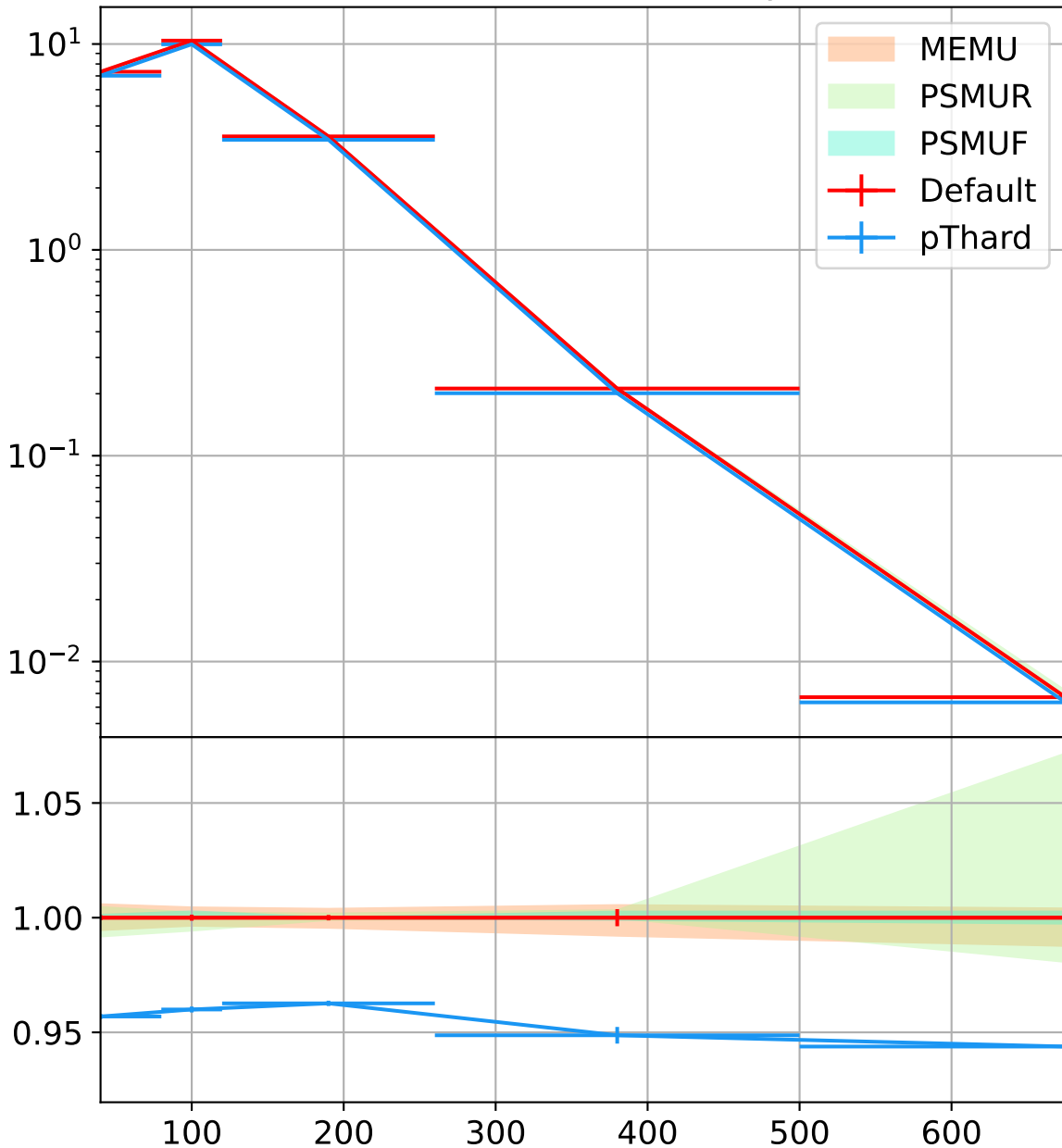
HISTO-PTH-NJETS-2-PTJ-30, Sherpa default PS
