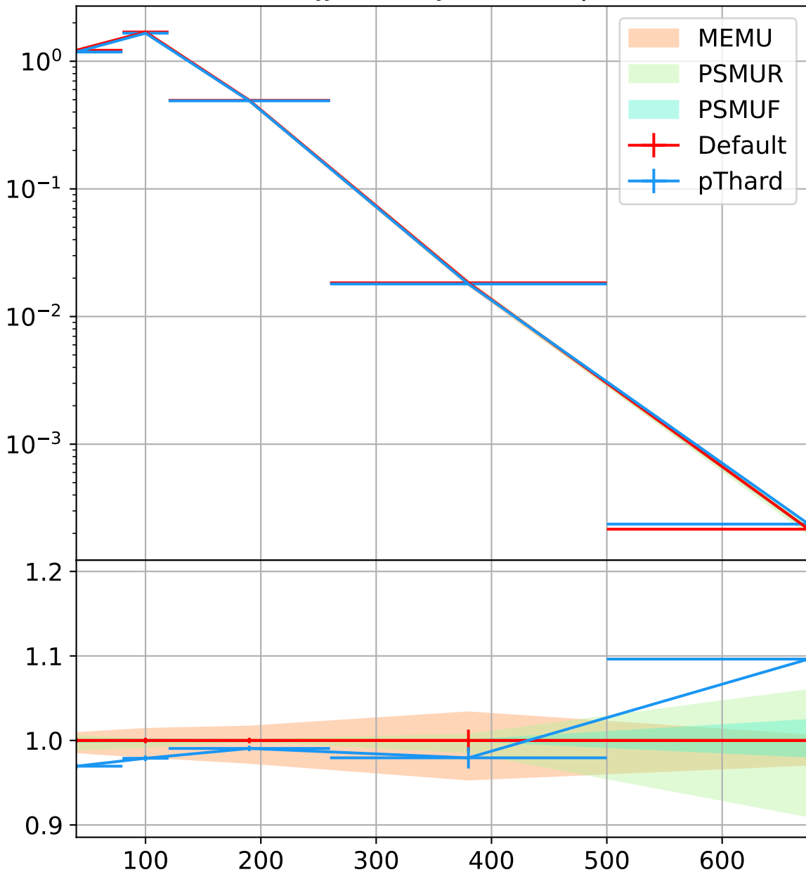
HISTO-PTH-DYJJ-6-7-PTJ-30, Sherpa default PS
