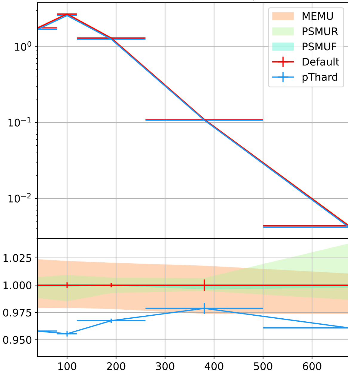
HISTO-PTH-DYJJ-2-4-PTJ-30, Sherpa default PS
