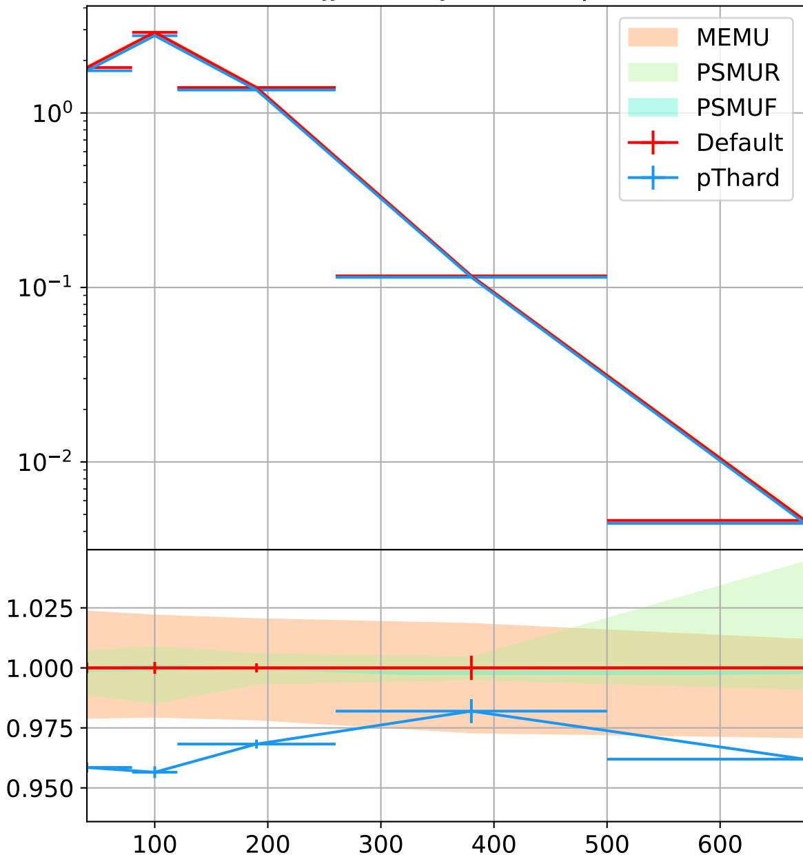
HISTO-PTH-DYJJ-2-4-PTJ-20, Sherpa default PS
