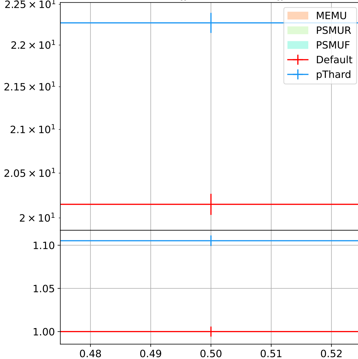
STXS-MJJ-700-1000-PTH-0-200-PTHJJ-25-INFTY-DPHJJ-0-Plov2, Sherpa default PS
