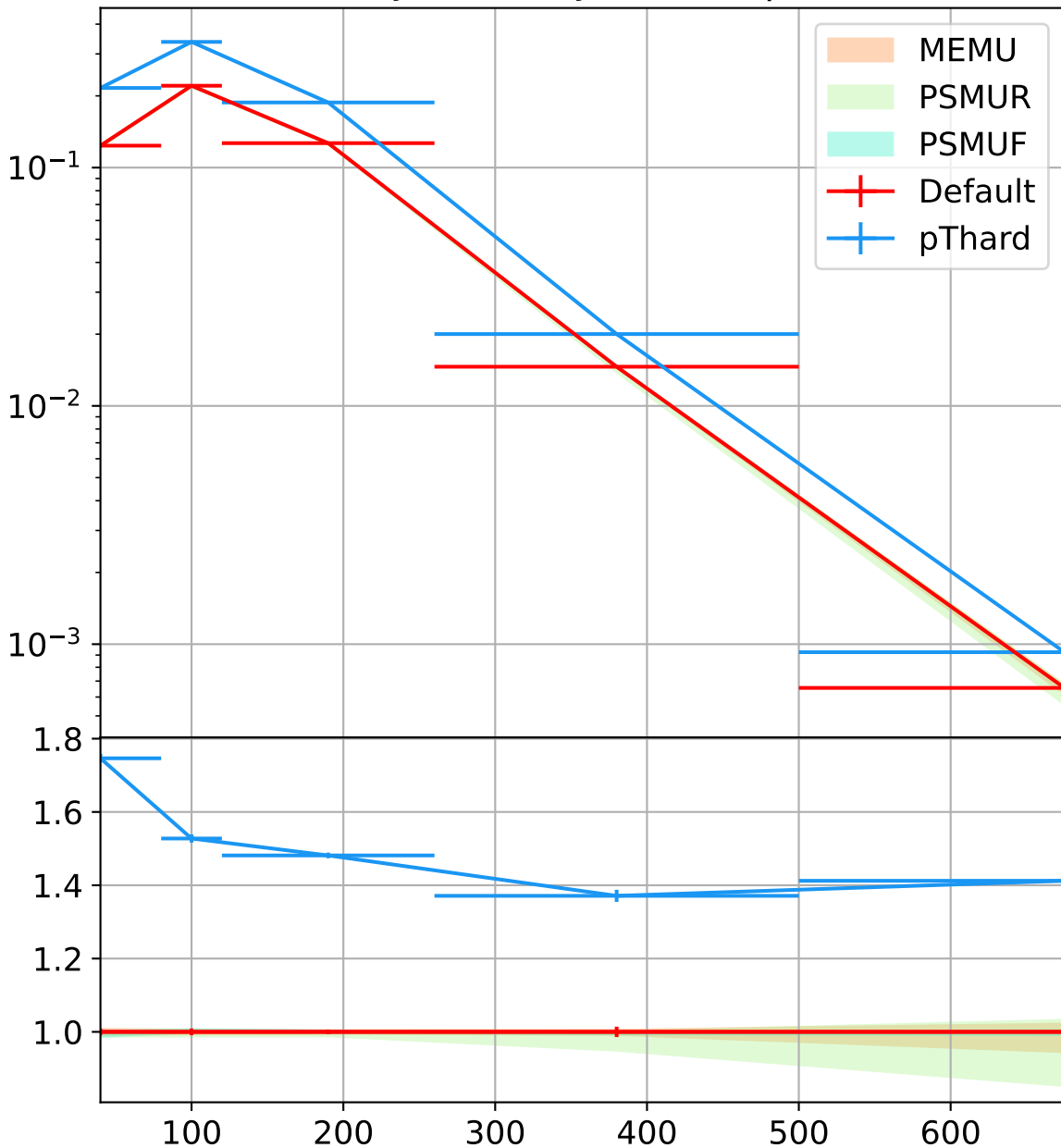
HISTO-PTH-NJETS-4-PTJ-20, Sherpa default PS
