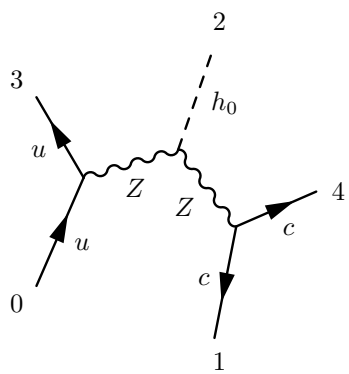
Graph 1 \mathcal{O}(g_s^0 g^3)
