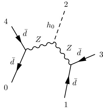
Graph 2 \mathcal{O}(g_s^0 g^3)
