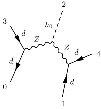
Graph 1 \mathcal{O}(g_s^0 g^3)
