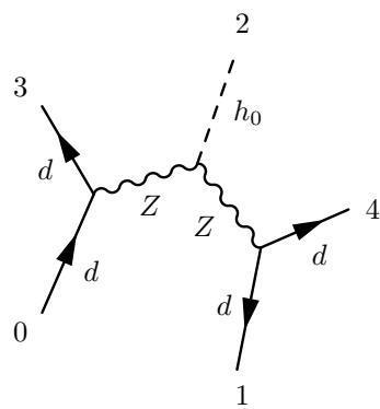
Graph 2 \mathcal{O}(g_s^0 g^3)
