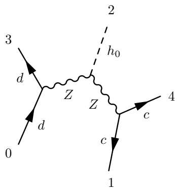
Graph 1 \mathcal{O}(g_s^0 g^3)
