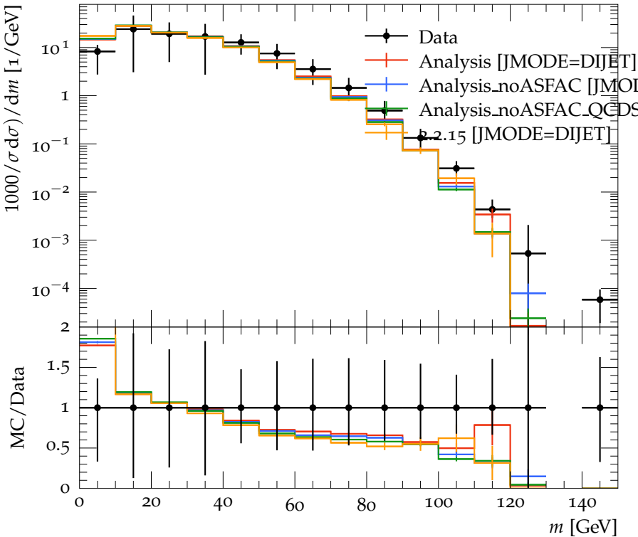
Pruned AK7 dijets, (p_T^1 + p_T^2)/2 = 220\text{--}300 GeV
