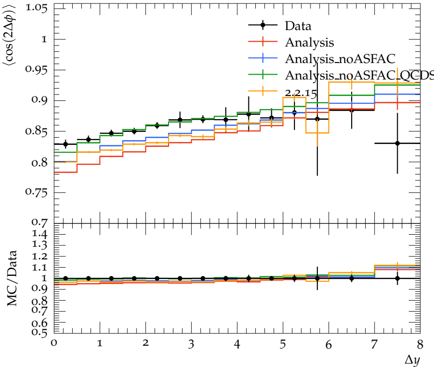
\langle \cos(2\Delta\phi) \rangle for gap events as a function of \Delta y
