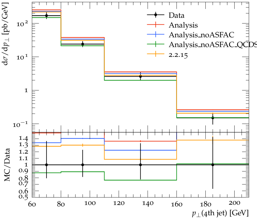
Transverse momentum of the 4th leading jet ( R = 0.4 )
