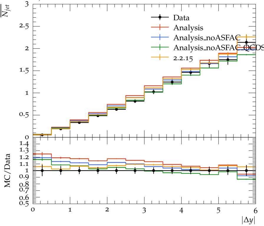
\overline{N_{jet}} vs |\Delta y| for 90 < \overline{P_T} < 120 , Fwd/Bwd
