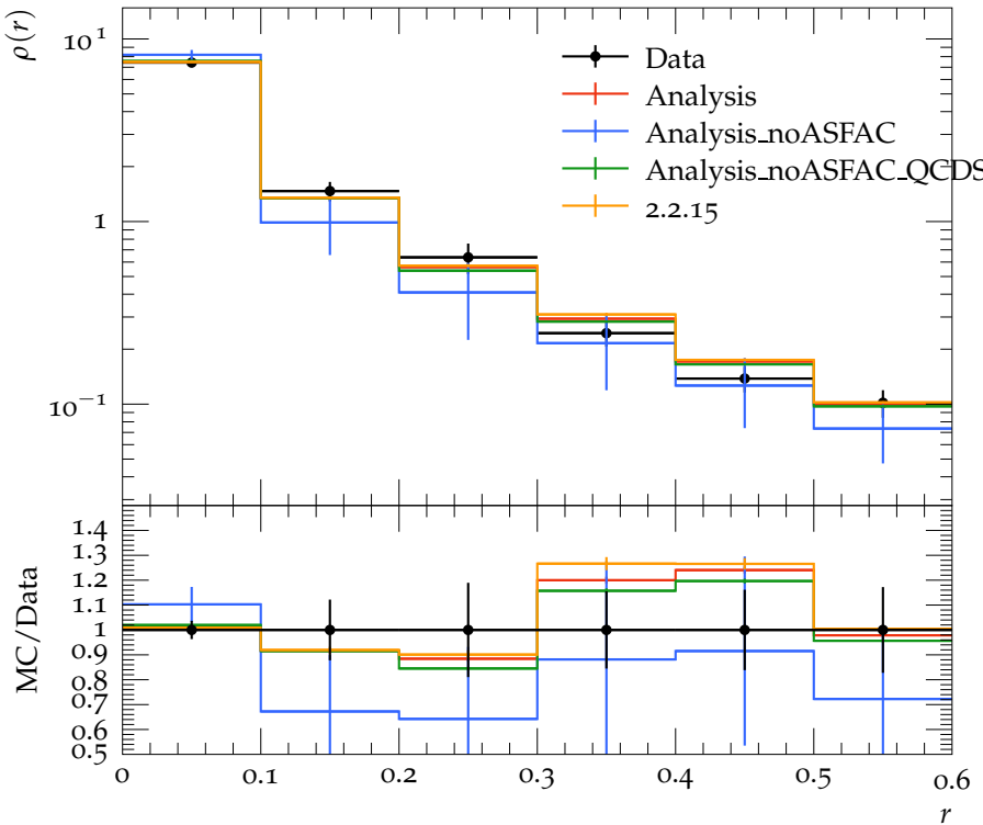
Jet shape \rho for p_{\perp} \in 400\text{--}500 GeV, y \in 0.0\text{--}0.3
