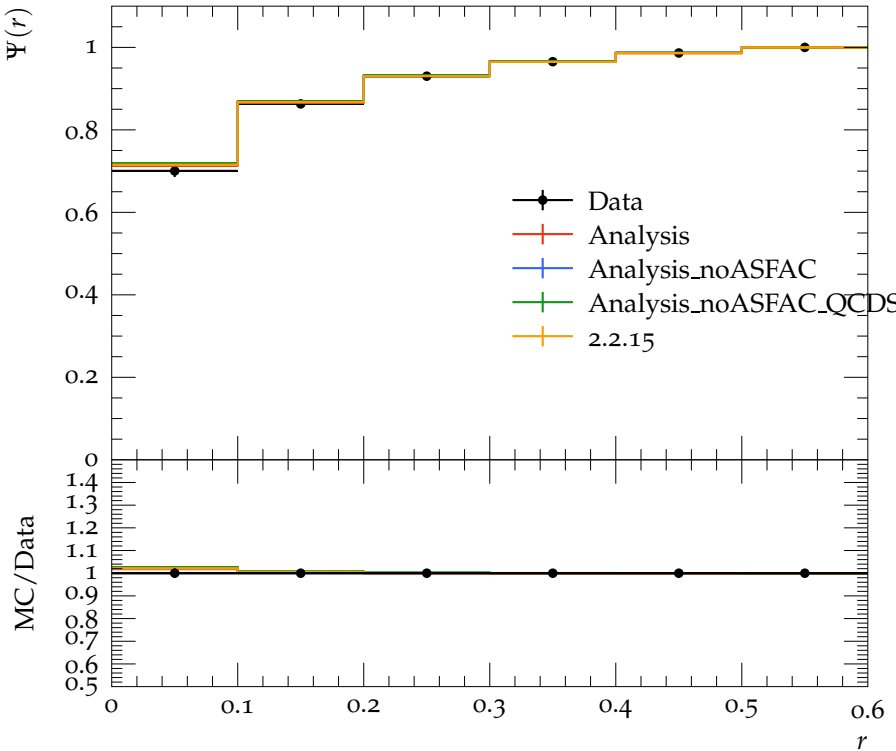
Jet shape \Psi for p_{\perp} \in 210\text{--}260 GeV, y \in 0.0\text{--}2.8
