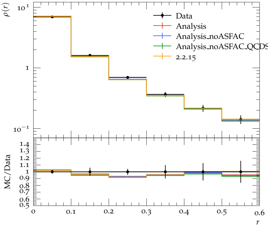
Jet shape \rho for p_{\perp} \in 210\text{--}260 GeV, y \in 0.8\text{--}1.2
