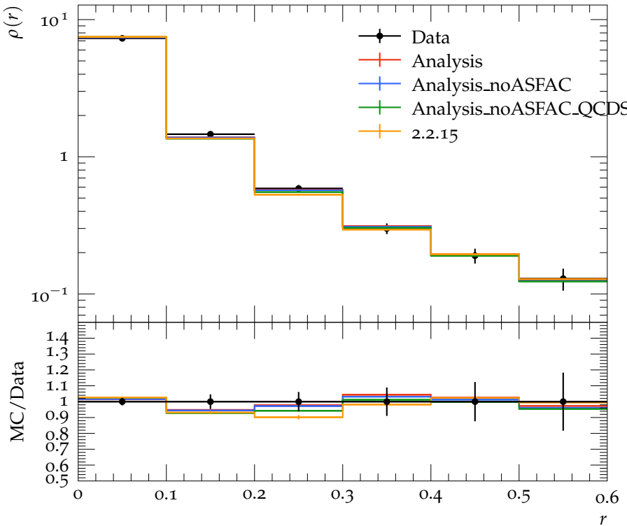
Jet shape \rho for p_{\perp} \in 160\text{--}210\text{ GeV} , y \in 2.1\text{--}2.8
