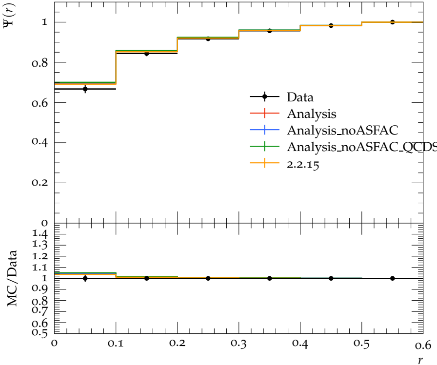
Jet shape \Psi for p_{\perp} \in 110\text{--}160\text{ GeV} , y \in 2.1\text{--}2.8
