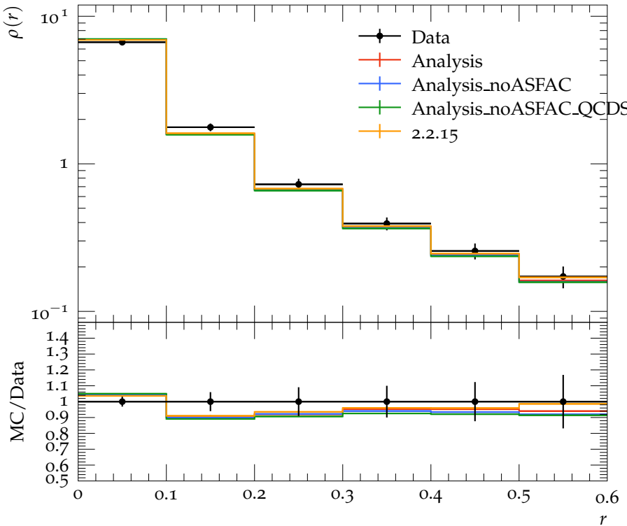
Jet shape \rho for p_{\perp} \in 110\text{--}160 GeV, y \in 2.1\text{--}2.8
