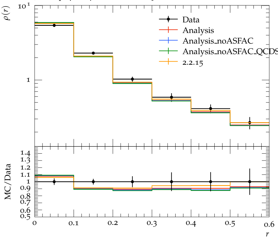
Jet shape \rho for p_{\perp} \in 60\text{--}80\text{ GeV} , y \in 2.1\text{--}2.8
