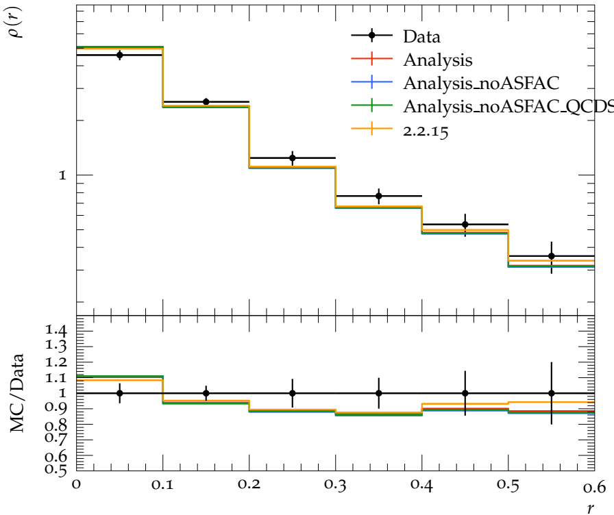
Jet shape \rho for p_{\perp} \in 40\text{--}60\text{ GeV} , y \in 2.1\text{--}2.8
