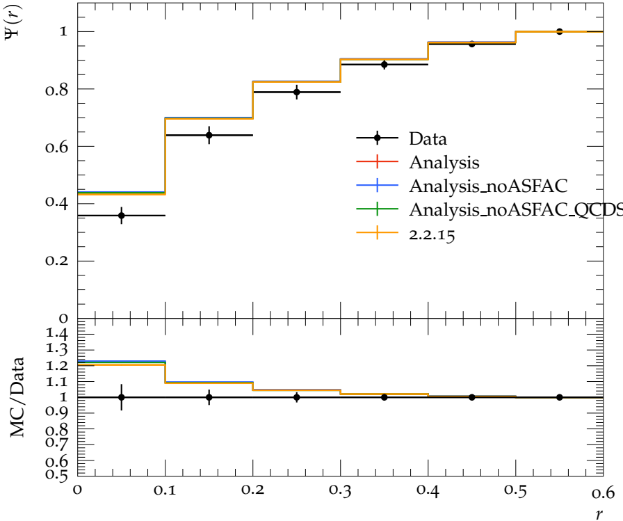
Jet shape \Psi for p_{\perp} \in 30\text{--}40\text{ GeV} , y \in 2.1\text{--}2.8
