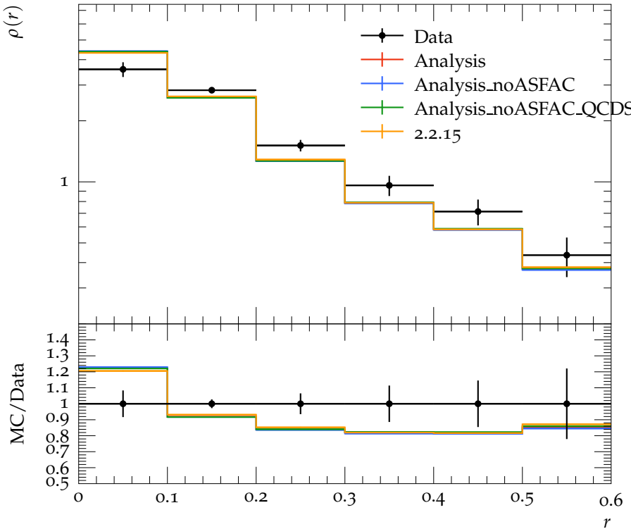
Jet shape \rho for p_{\perp} \in 30\text{--}40\text{ GeV} , y \in 2.1\text{--}2.8
