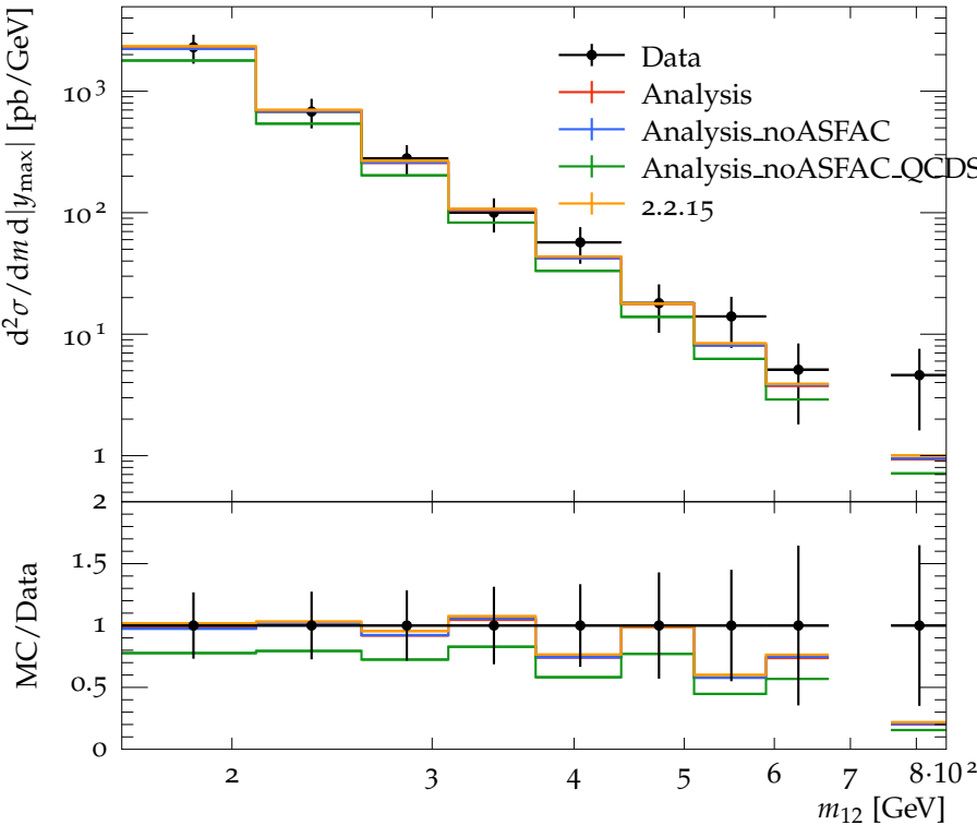
Dijet mass spectrum for 0.3 < |y_{\max}| < 0.8 . anti-KT, R = 0.4 .
