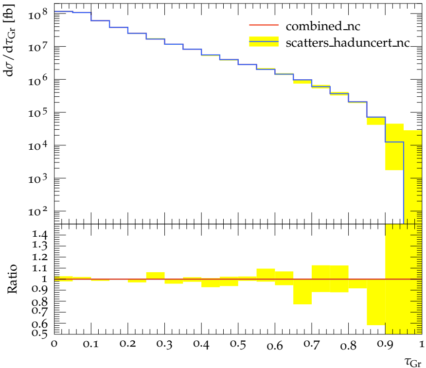
Groomed 1-jettiness \tau_{\text{Gr}} with z_{\text{cut}} = 1
