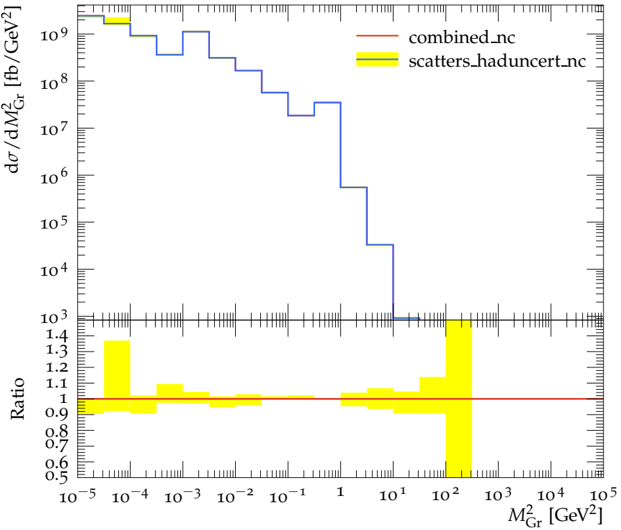
Groomed invariant mass M_{\text{Gr}}^2 with z_{\text{cut}} = 0.5
