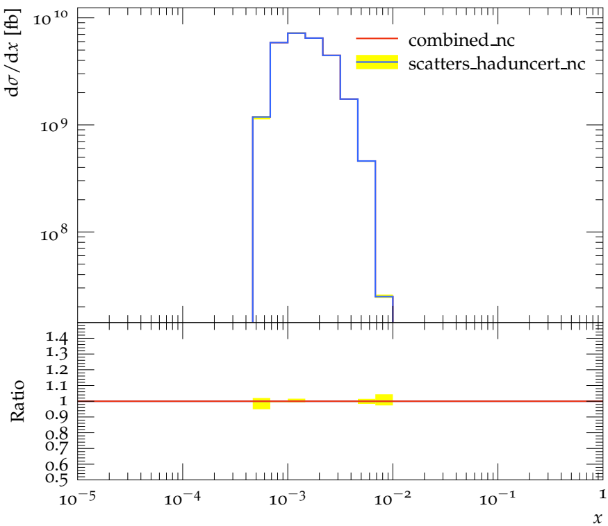
Distribution of Bjorken- x in bin of Q^2
