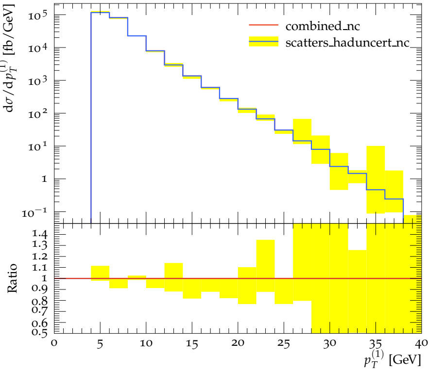
Distribution of leading jet transverse momentum in bin of Q^2
