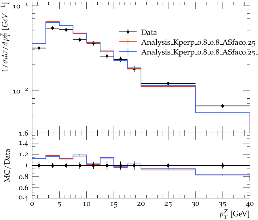
CMS, 8 TeV, Z boson p_T distribution in Di-muon channel
